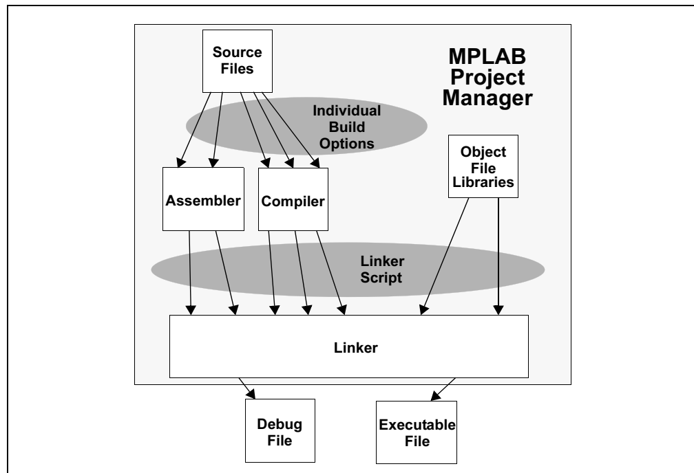
FIGURE 1-6: MPLAB PROJECT MANAGER
